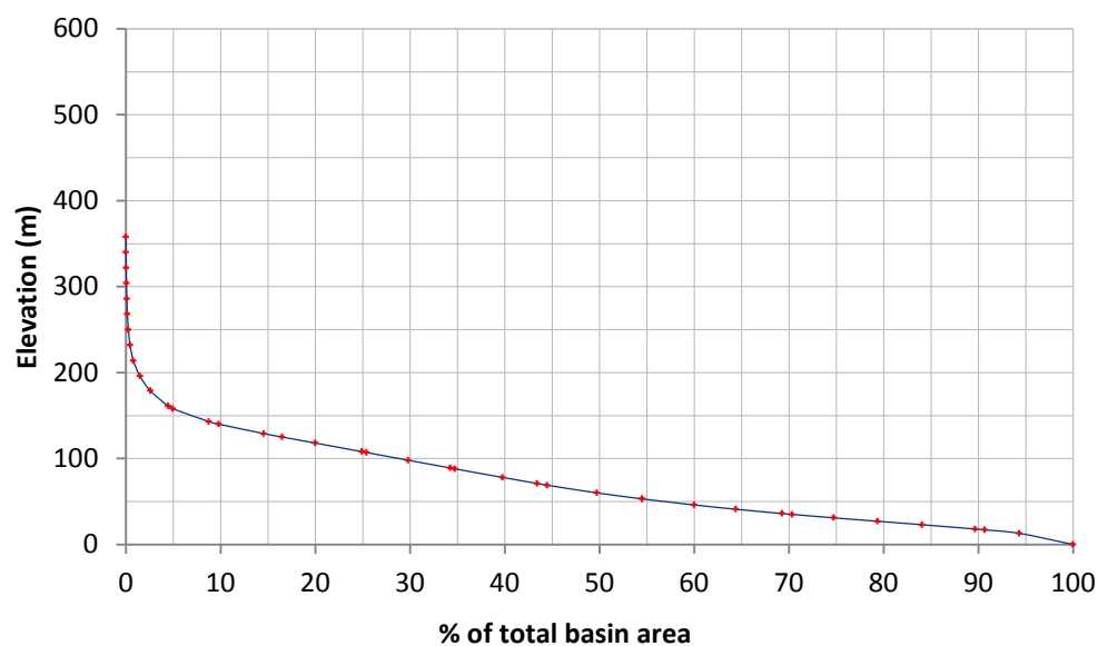
Hypsometric curve - Basin 14 Po-Joda
