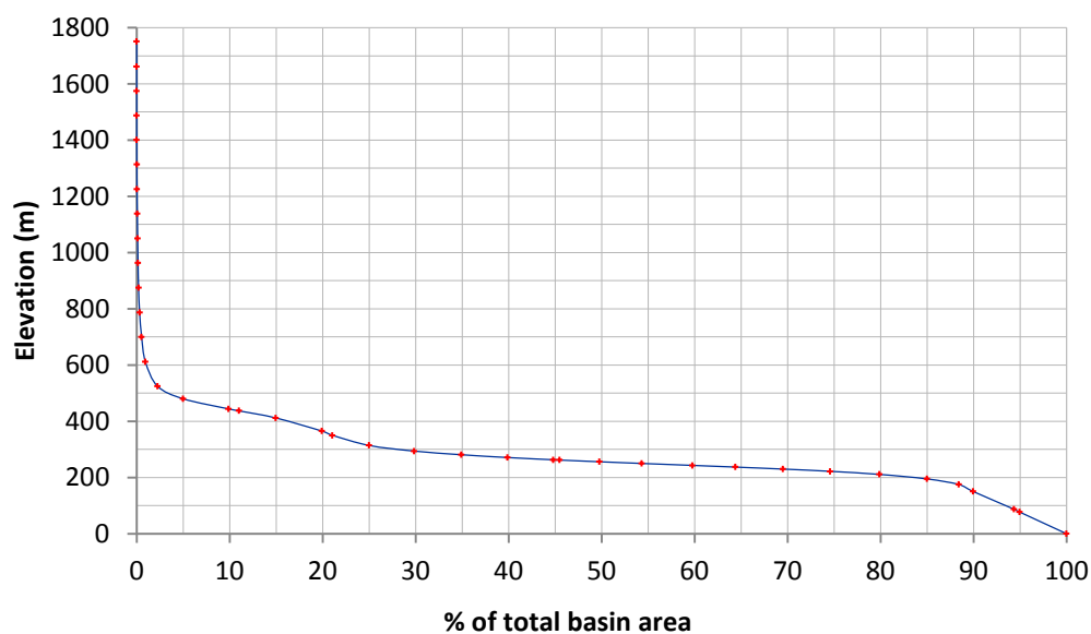
Hypsometric curve - Basin 06 St. John
